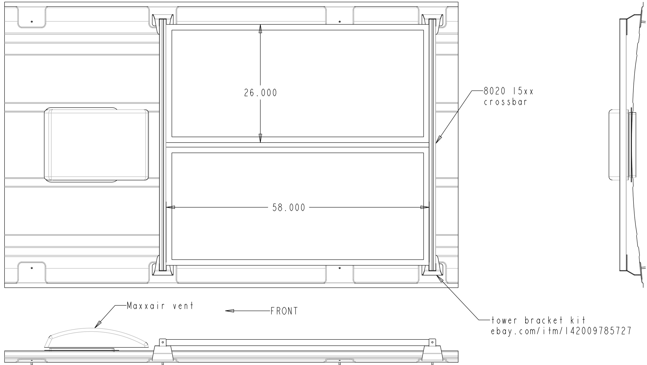
Transit 148 with 2x160 watt & forward vent location SCALE 0.100 Contact Info: Heinvs@Impact3d.com 541 490 5098
